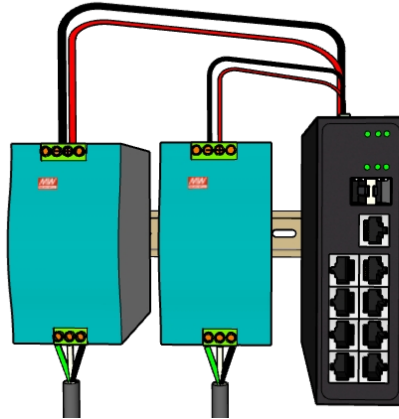
DIN Mounted with x2 PS-48v480w
