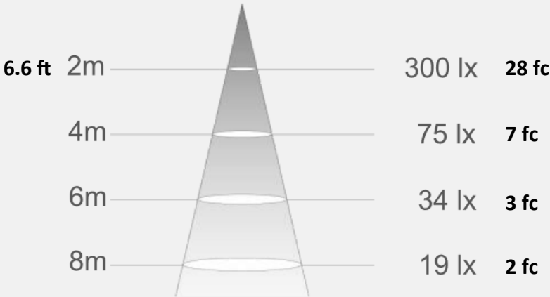
Illuminance (lx)
