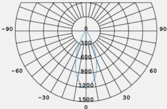
Light Distribution
