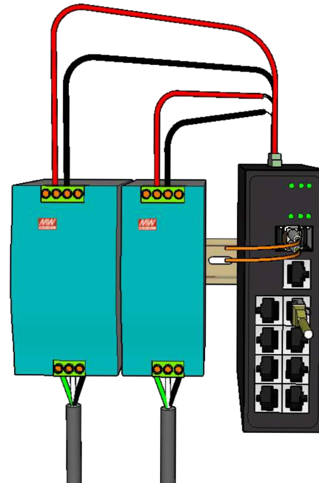
DIN Mounted with PS-48v480w and PS-48v240w
