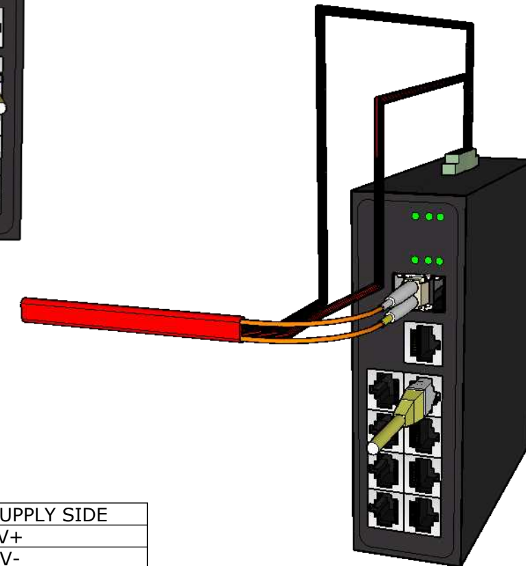
Wall Mounted with Remote Power
