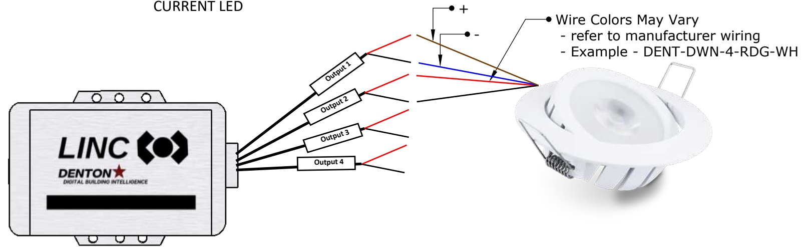
COLOR TUNABLE WARM/COOL CONSTANT CURRENT LED
