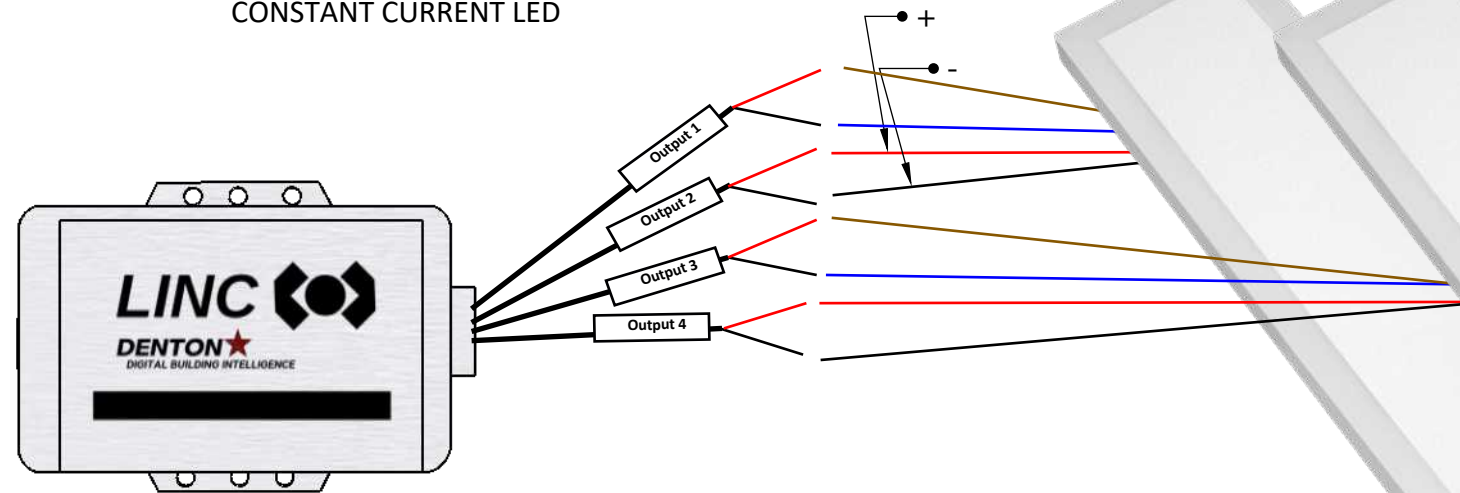
COLOR TUNABLE WARM/COOL CONSTANT CURRENT LED
